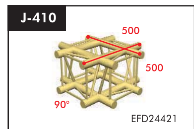
4-way cross 90° Weight: 4.50 kg Price: € 398.70
