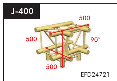
4-way T-joint 90° Weight: 4.50 kg Price: € 398.70
