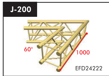
2-way corner 60° Weight: 5.30 kg Price: € 253.50
