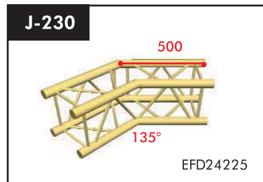
2-way corner 135° Weight: 2.90 kg Price: € 225.50
