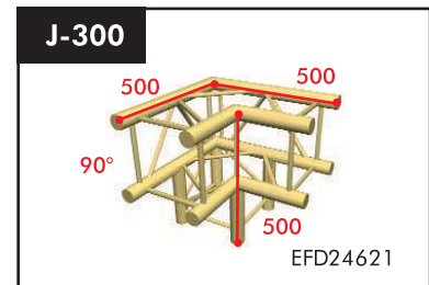
3-way corner 90° Weight: 4 kg Price: € 291.70
