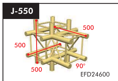
5-way T-joint 90° Weight: 5 kg Price: € 479
