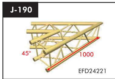
2-way corner 45° Weight: 3.50 kg Price: € 253.50
