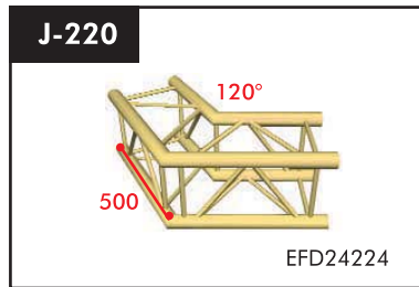
2-way corner 120° Weight: 2.90 kg Price: € 225.50
