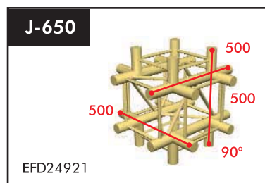
6-way T-joint 90° Weight: 5.30 kg Price: € 524.90
